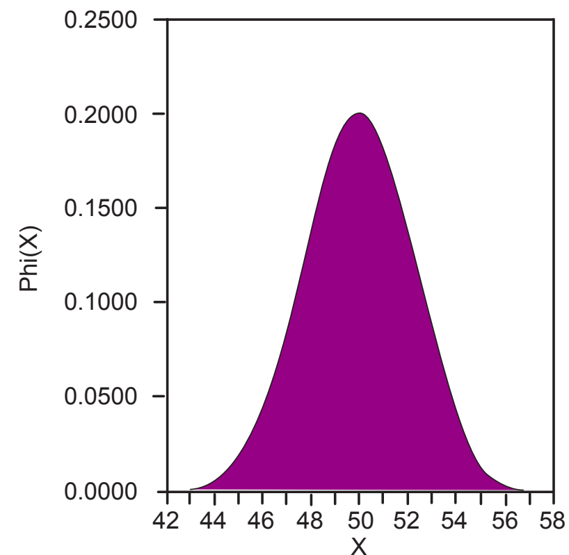
Figure 2. A normal distribution with \mu = 50 and \sigma = 2 .
