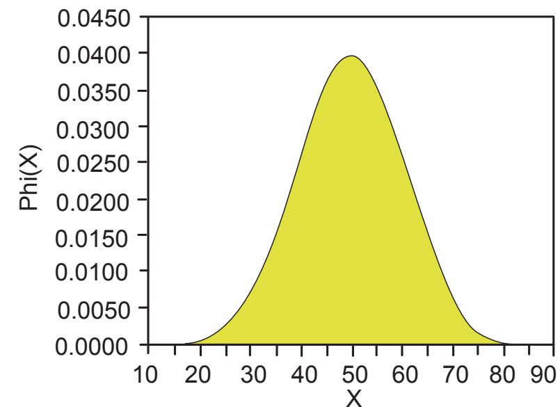
Figure 1. A normal distribution with \mu = 50 and \sigma = 10 .
