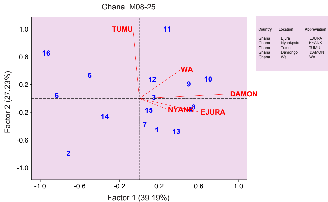
Figure 15. SREG Biplot of Intermediate/Late Maturing DT Variety Trial evaluated at five sites in Ghana in 2008.
