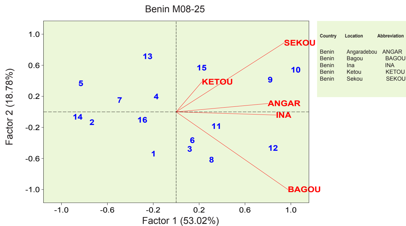
Figure 14. SREG Biplot of Intermediate/Late Maturing DT Variety Trial evaluated at 5 sites in Bénin in 2008.
