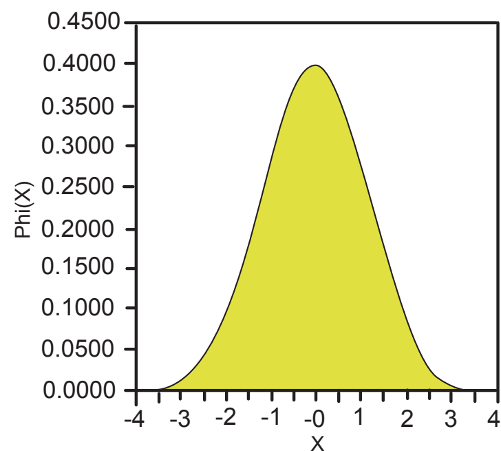
Figure 3. The Standard Normal Distribution; \mu = 0, \sigma = 1 .
